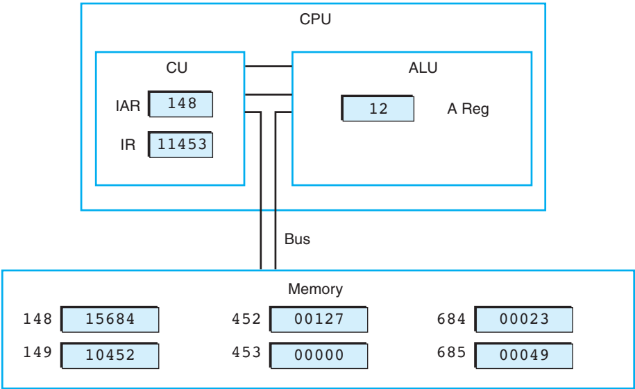
FIGURE A.2 Instruction processing
