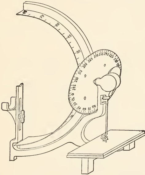
FIG. 9. Perimeter for Mapping the Retinal Zones.
