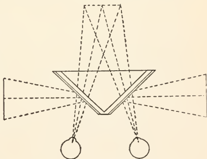
FIG. 49. Plan of Wheatstone's Stereoscope.
