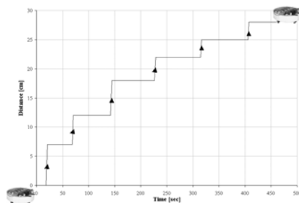
Fig. 7. Average charge/discharge cycles shown with respect to time and space
