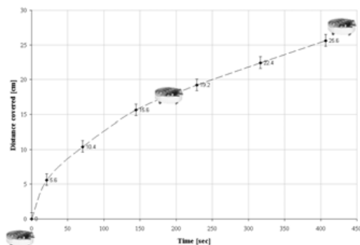
Fig. 8. Progression of EcoBot I along flat surface
