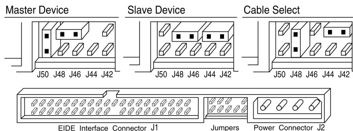
Real View of Maxtor Hard Drive Master, Slave and cable Select Settings
