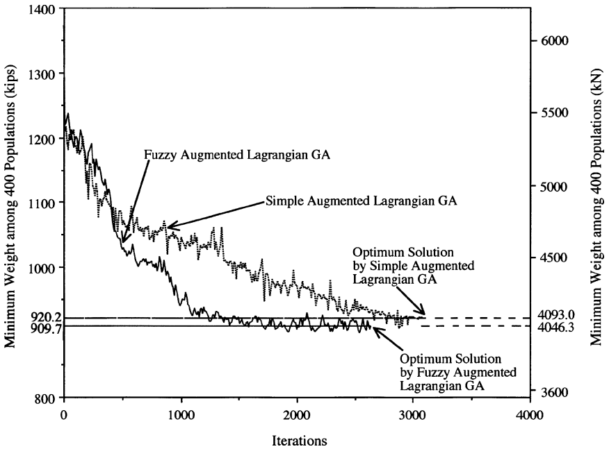
Figure 4.10 Iteration history of the 1310-member space truss
