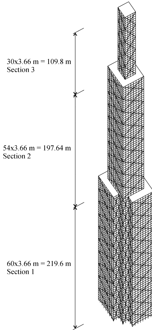
Figure 7.8 A 144-story steel space moment-resisting frame structure (Park and Adeli, 1997a)
