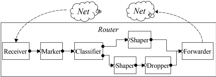
Fig. 1. Router Configuration
