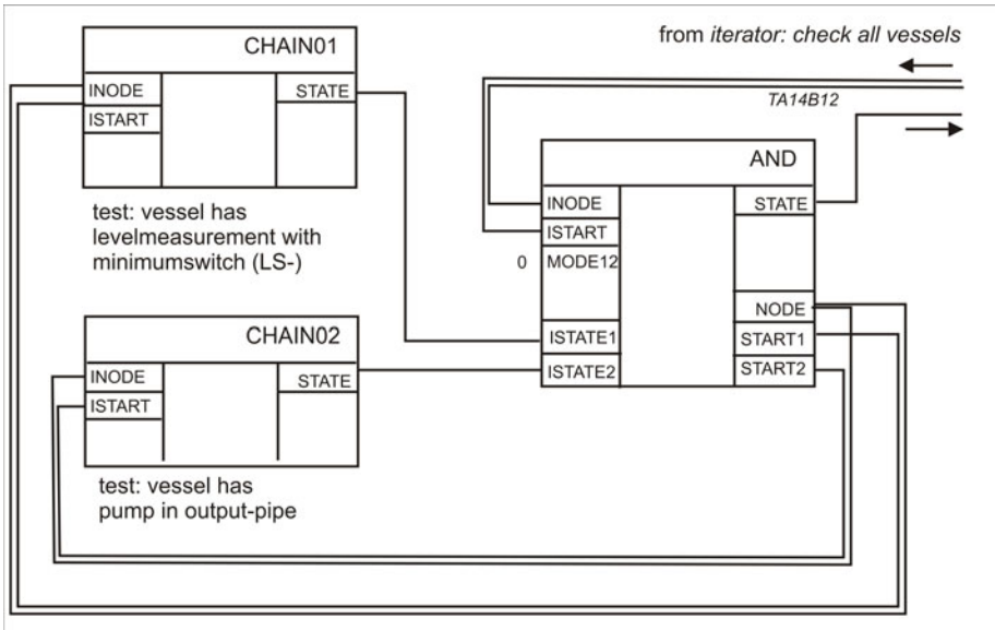
Fig. 12. Formulating rules as function-block networks
