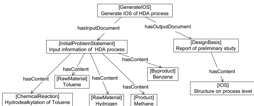
Fig. 10. Example of a conceptual design step on the instance level
