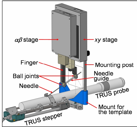
Fig. 1. CAD model of the parallel robot mounted over the TRUS probe on the mounting posts of the template
