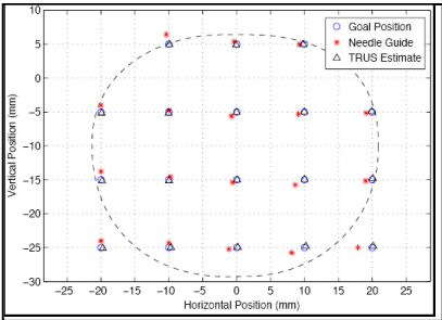
Fig. 6. Accuracy of robotically guided needle insertion relative to TRUS
