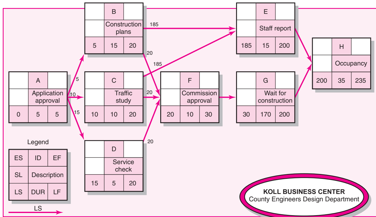
FIGURE 6.7 Activity-on-Arrow Network Backward Pass
