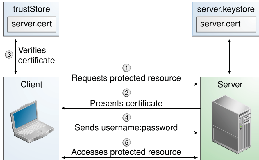
FIGURE 24-5 User Name/Password-Based Mutual Authentication
