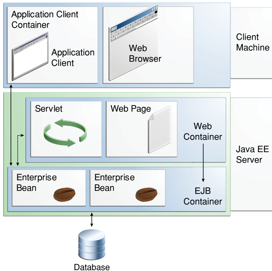
FIGURE 25-1 Java EE Server and Containers
