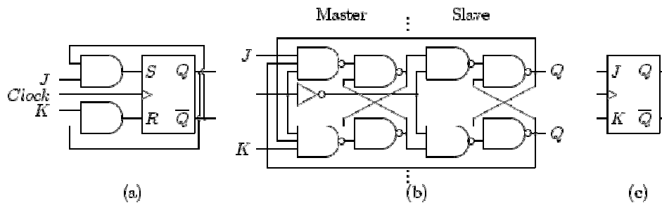
Figure 2.9: JK flip flop
