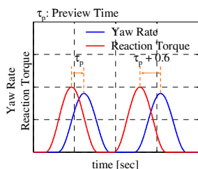
Fig. 8. Example of Changing the Preview Time
