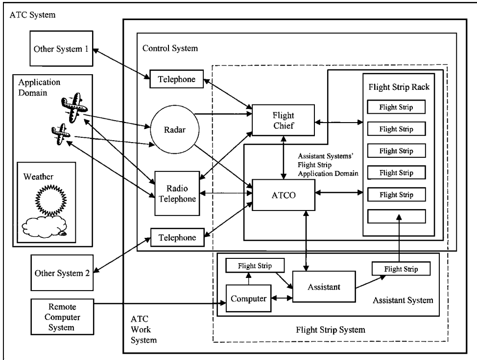
FIG. 1.4. A simplified model of a traditional air traffic control (ATC) system that uses paper-based flight strips.
