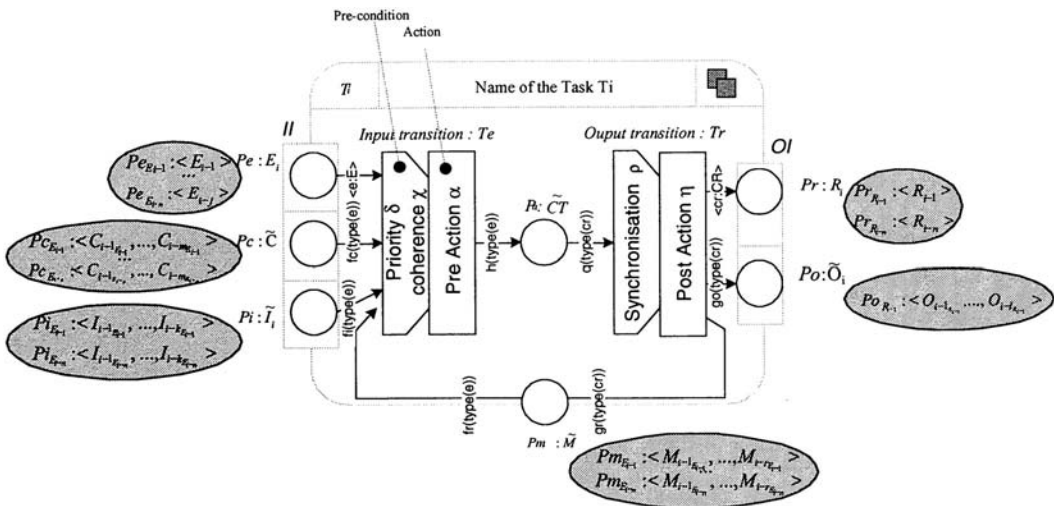
FIG. 25.4. Task control structure (TCS).
