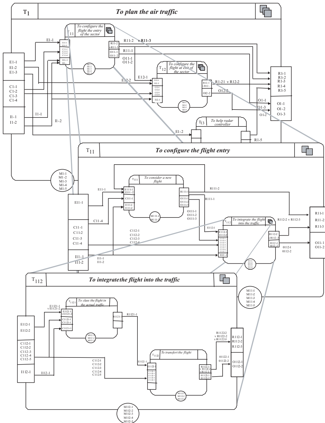
FIG. 25.3. Graphical specification of the task class "T 1 : Schedule the traffic" (structural model).
