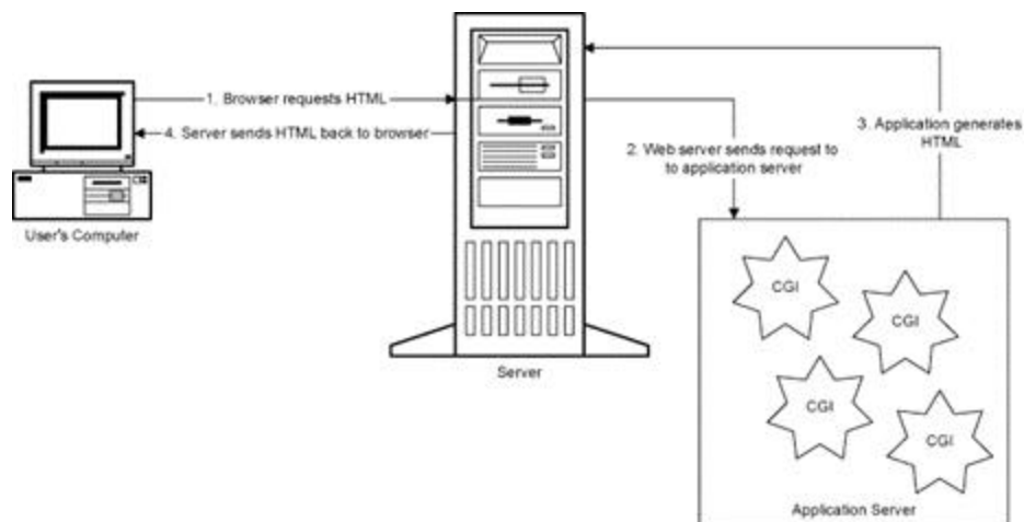
Figure 1.5. An application server.
