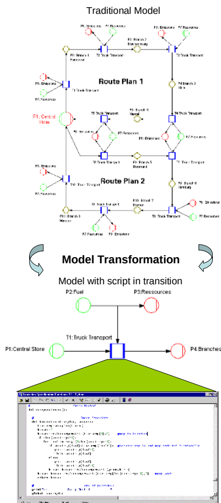
Figure 3. Transforming a material flow network for optimisation purposes
