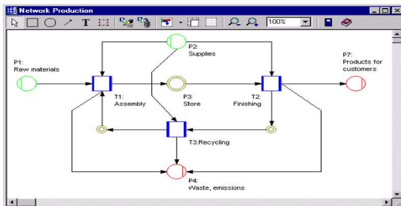
Figure 1. Structure of a simple material flow network
